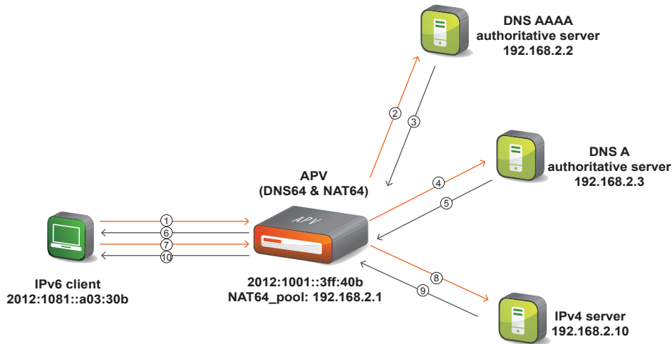
Figure 1-1 "IPv6 to IPv4" Application Scenario
