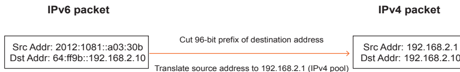
Figure 1-2 NAT64 Address Translation
